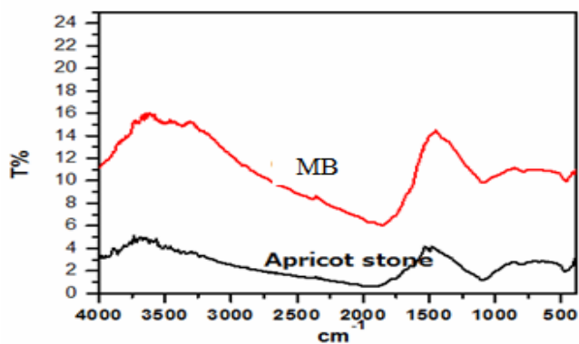
Fig. 2: FT-IR spectra for adsorption of MB on the surface of Apricot stone.
